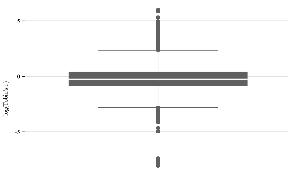
Appendix 2: Box Plot of Log Tobin's q
